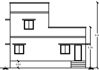
ELEVATION (SCALE 1:100)
