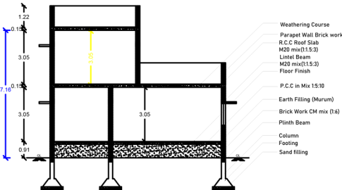
SECTION "A-A" (SCALE 1:100)
