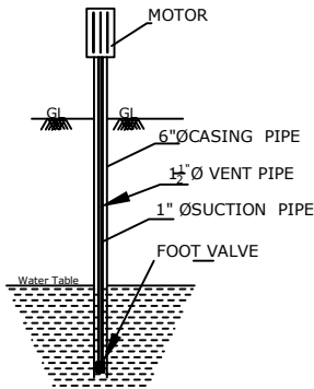
SEC. OF BOREWELL
