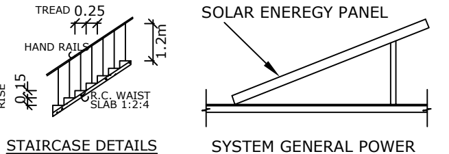
STAIRCASE DETAILS
