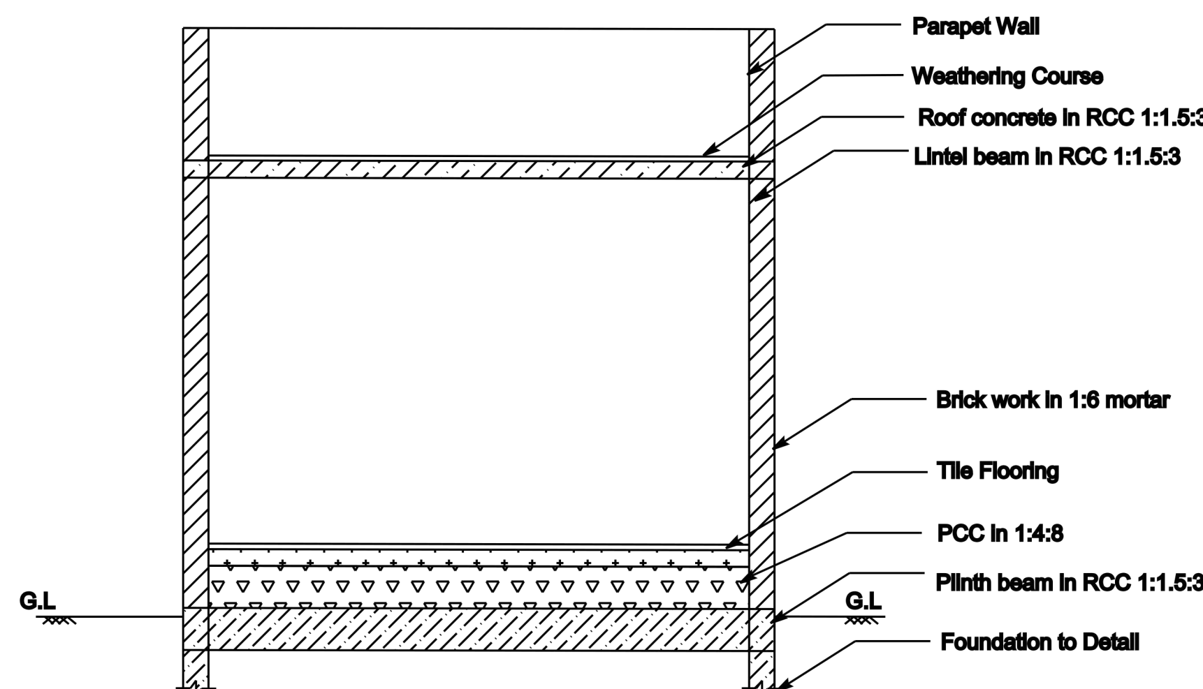
SECTION BB
