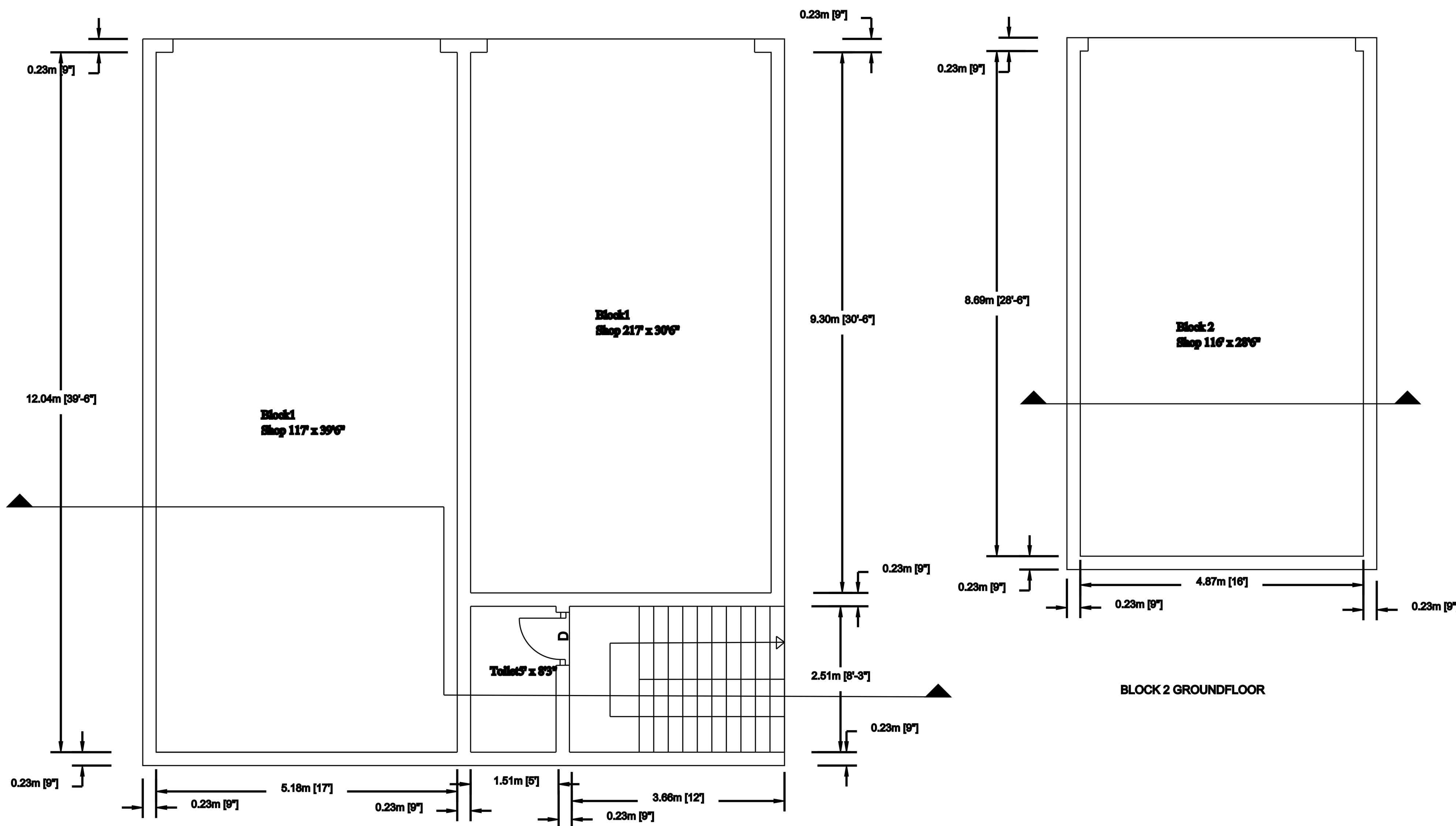
BLOCK 1 GROUND FLOOR
