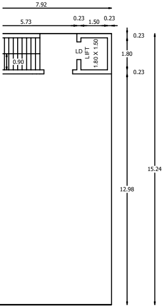
SILT FLOOR PLAN
