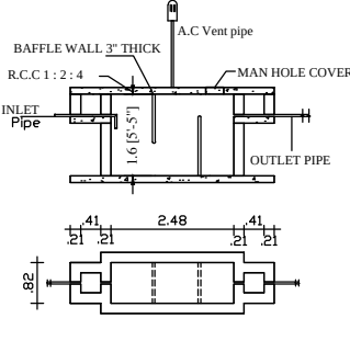
SEPTIC TANK
