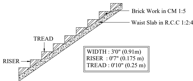
STAIRCASE DETAILS
