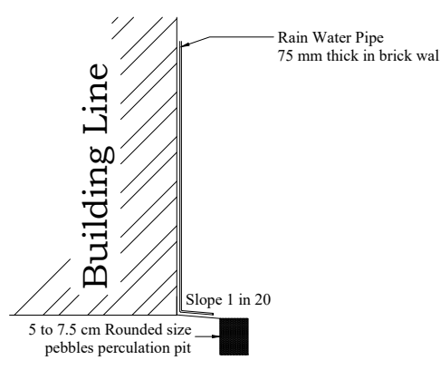
RAINWATER HARVESTING
