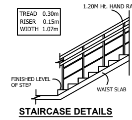
STAIRCASE DETAILS
