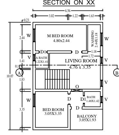
PROPOSED BUILDING OF FIRST FLOOR
