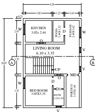
PROPOSED BUILDING OF GROUND FLOOR
