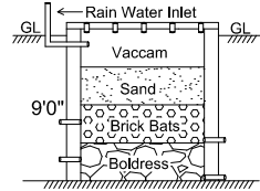
RAIN WATER HARVESTING TANK
