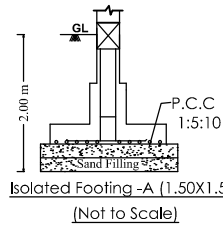
FOUNDATION DETAIL - A
