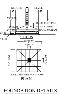
FOUNDATION DETAILS
