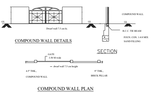
COMPOUND WALL PLAN
