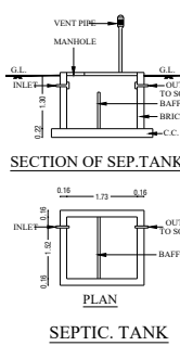
SEPTIC TANK
