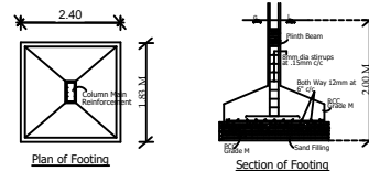
FOUNDATION DETAILS
