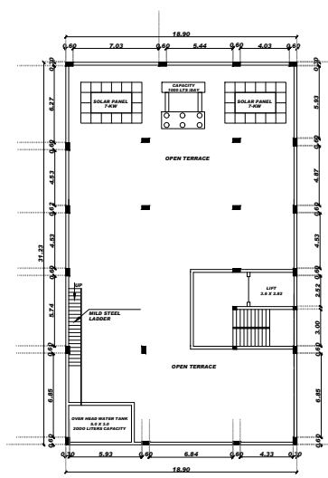
PROPOSED HEAD ROOM AND OPEN TERRACE FLOOR PLAN
