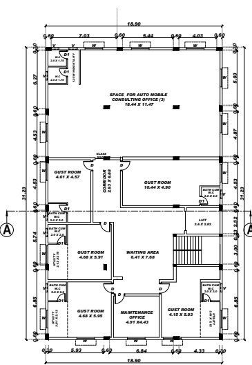
PROPOSED SECOND FLOOR PLAN
