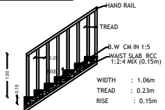
STAIRCASE DETAILS :-
