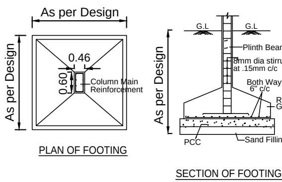
FOUNDATION DETAILS
