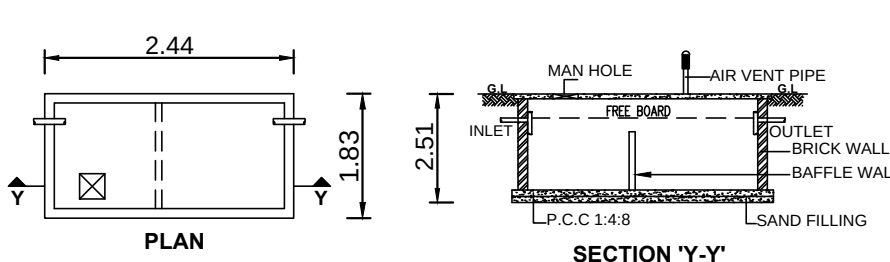
SEPTIC TANK DETAILS
