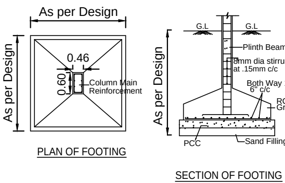
FOUNDATION DETAILS
