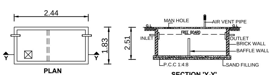
SEPTIC TANK DETAILS
