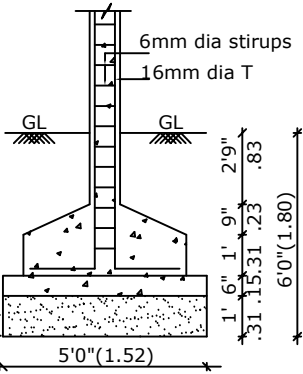
COLUMN FOUNDATION DETAIL
