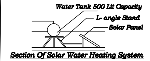
Section Of Solar Water Heating System
