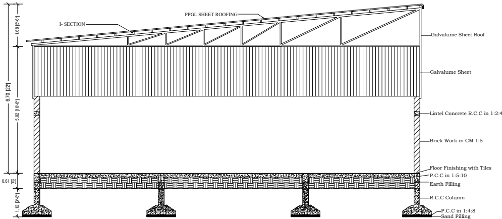
SECTION X-X
