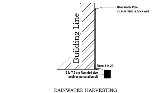
RAINWATER HARVESTING
