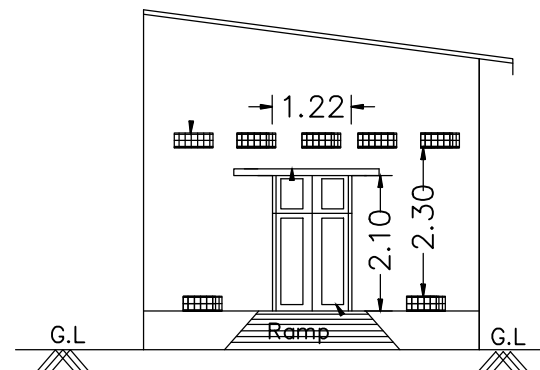
FRONT ELEVATION
