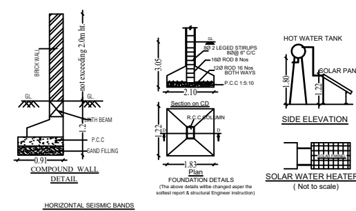
HORIZONTAL SEISMIC BANDS
