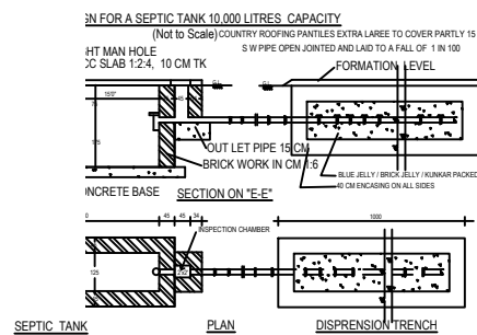
SEPTIC TANK PLAN DISPERNSION TRENCH
