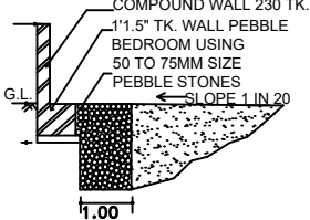
RAIN WATER HARVESTING TRENCH
