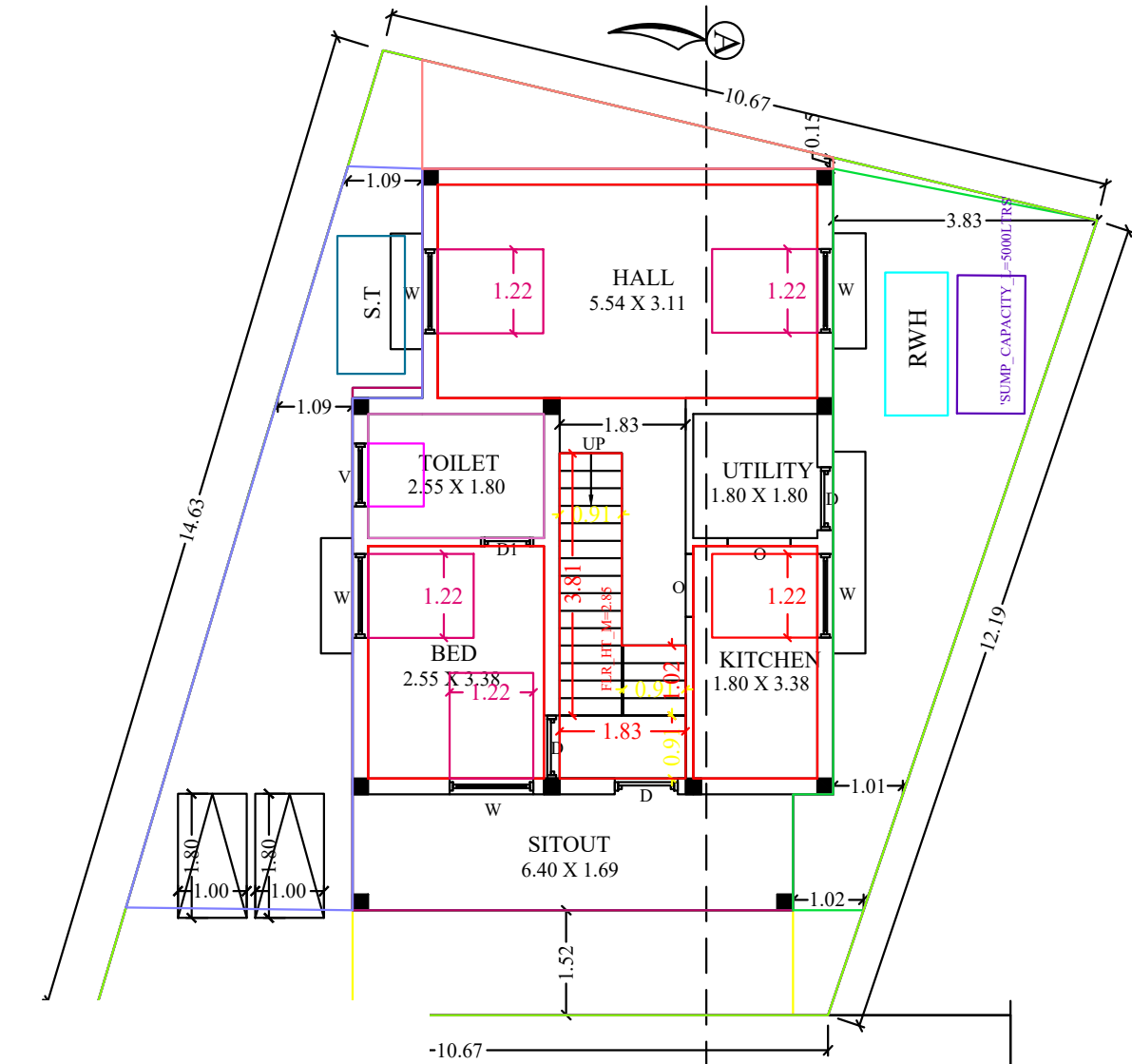
ID FLOOR PLAN
