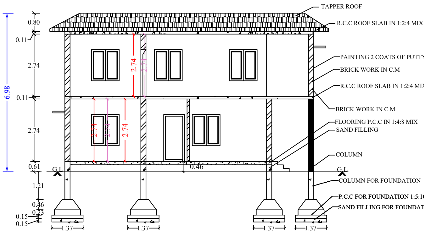
SECTION ON-AA
