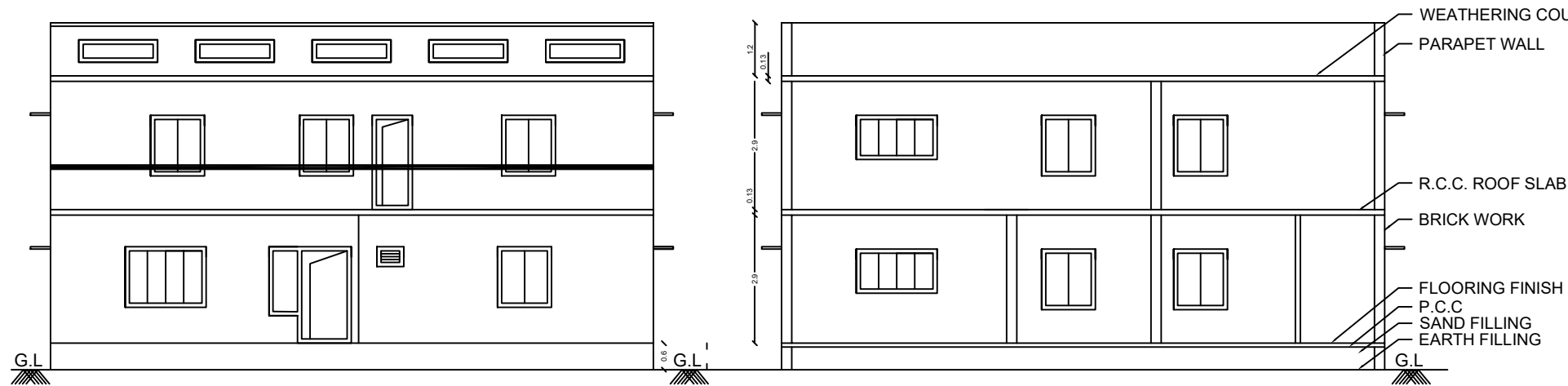
FRONT ELEVATION
