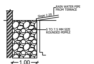
INWATER HARVESTING TRENCH
