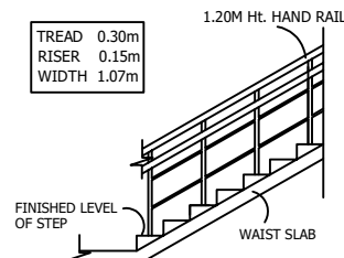
STAIRCASE DETAILS
