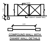
COMPOUND WALL WITH DWARF WALL DETAILS
