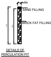
DETAILS OF PERCOLATION PIT
