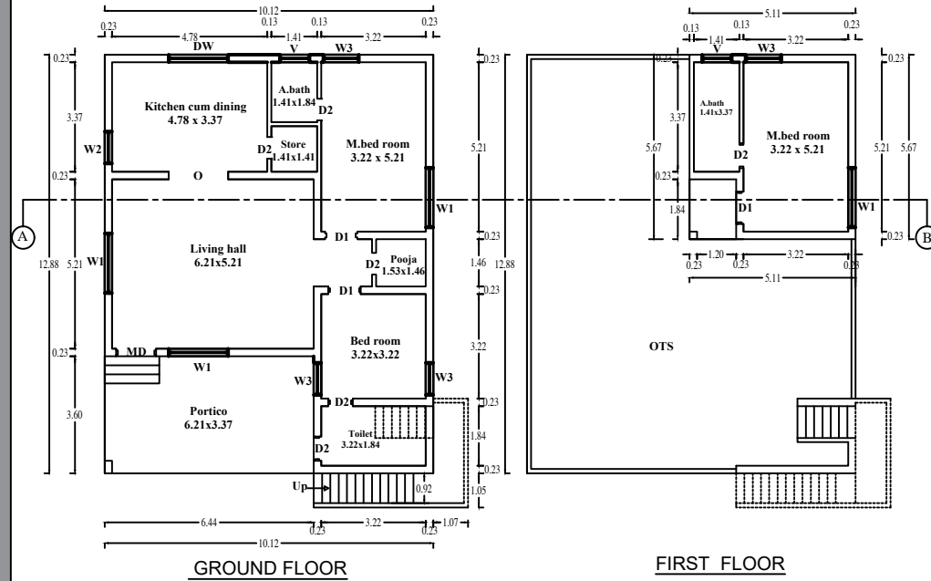
GROUND FLOOR
