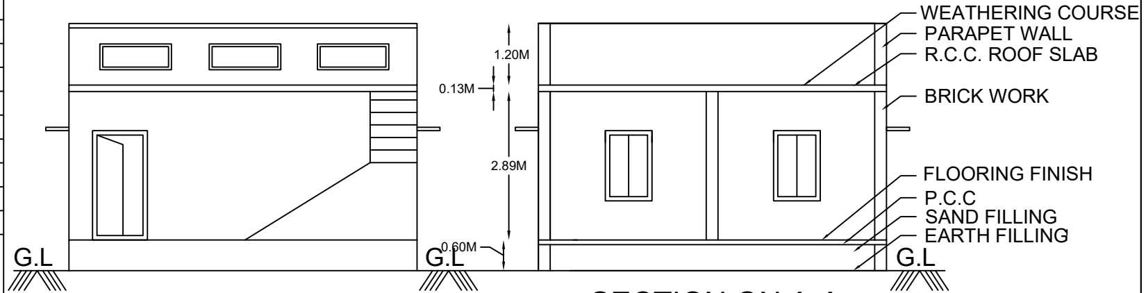
FRONT ELEVATION
