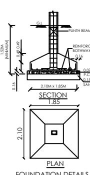
FOUNDATION DETAILS
