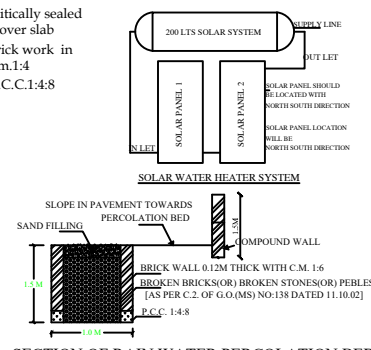
SECTION OF RAIN WATER PERCOLATION BED
