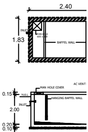
PLAN OF SEPTIC
