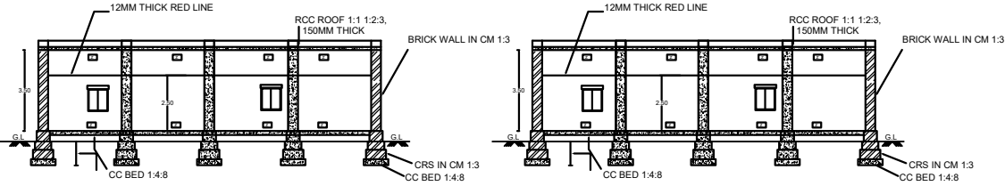
SECTION ON A-A
