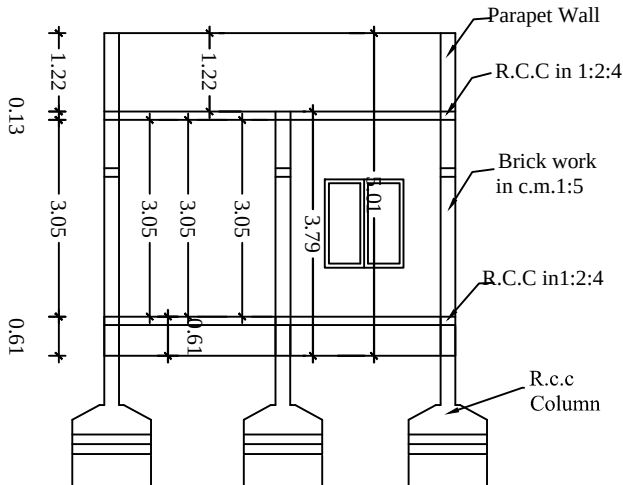
CROSS SECTION-AA
