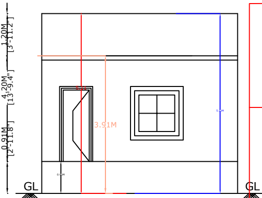
FRONT ELEVATION
