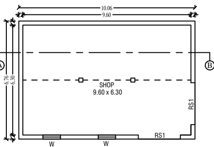
PROPOSED BUILDING IN GROUND FLOOR
