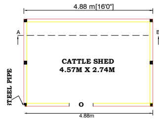
CATTLE SHED - PLAN
