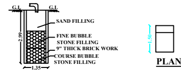
SECTION ON RAIN WATER COLLECTION TANK
