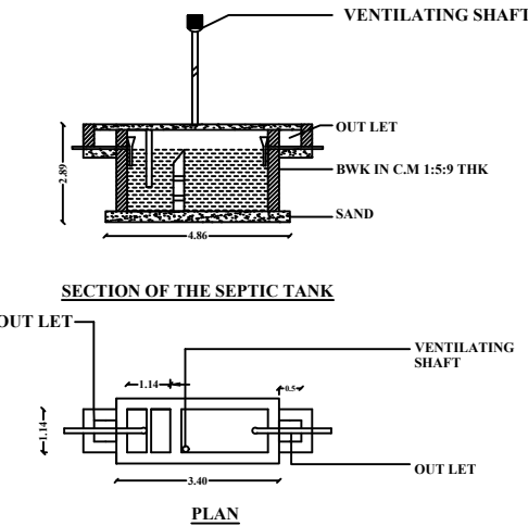
SEPTIC TANK
