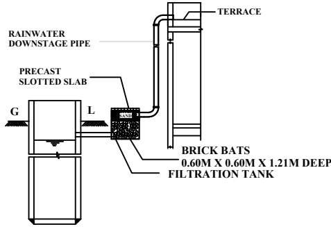
RAIN WATER COLLECTION TANK COLLECTION OF RAIN WATER FROM BUILDING
