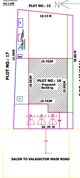
TE PLAN SCALE 1:100
