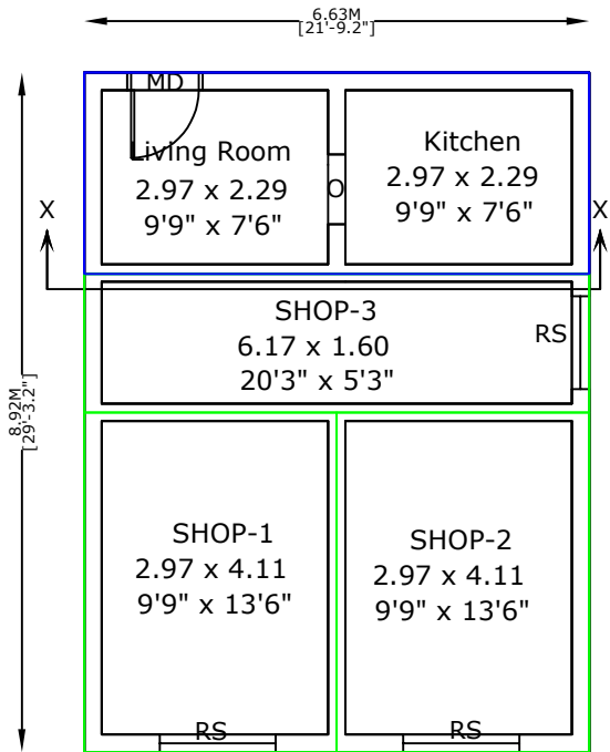
SITE CUM PRO.GROUND FLOOR
