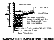
RAINWATER HARVESTING TRENCH
