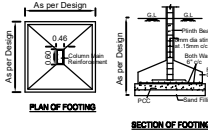
FOUNDATION DETAILS
