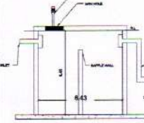
SEPTIC TANK
