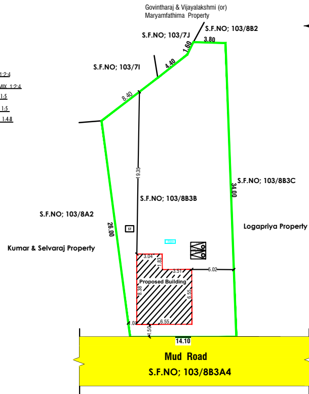
SITE PLAN
