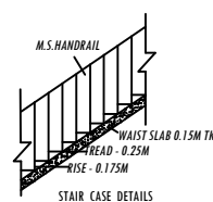
STAIR CASE DETAILS
