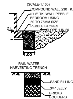
RAIN WATER COLLECTION TRENCH
