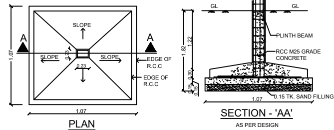
FOUNDATION DETAILS
