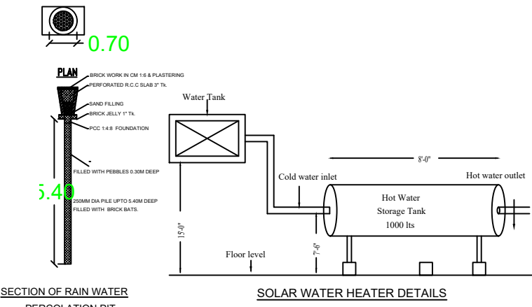
SECTION OF RAIN WATER PERCOLATION PIT
