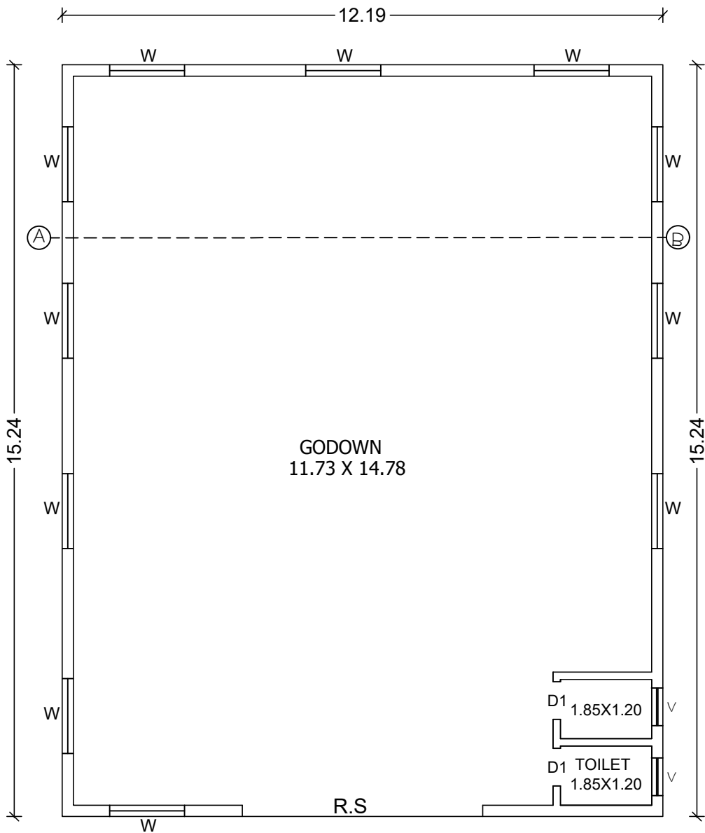
FLOOR PLAN I FACEING
