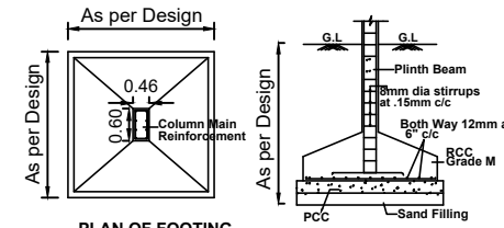
FOUNDATION DETAILS
