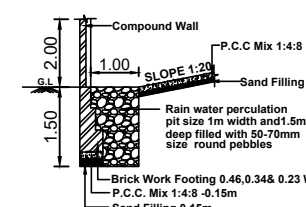
RAINWATER HARVESTING TRENCH
