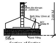
FOUNDATION DETAILS
