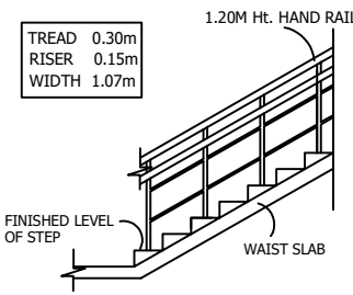
STAIRCASE DETAILS
