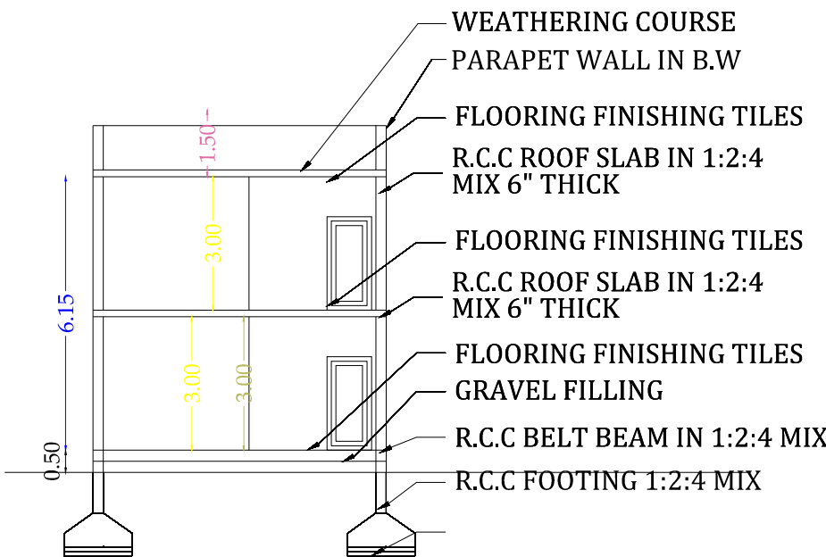
SECTION A TO B
