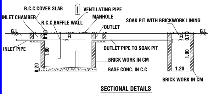
SECTIONAL DETAILS
