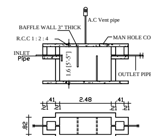
SEPTIC TANK
