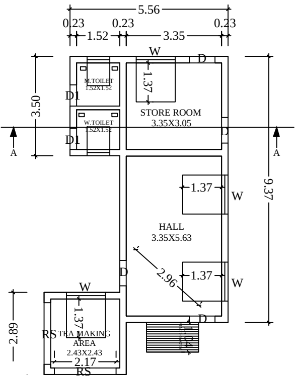
PLAN FOR GROUND FLOOR
