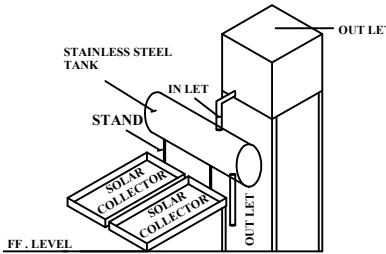
SOLAR HEATING WATER SYSTEM
