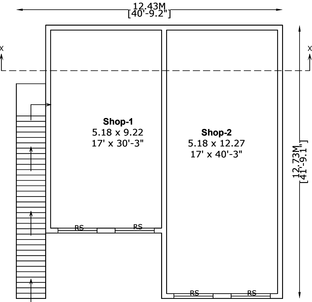
SITE CUM PRO.GROUND FLOOR
