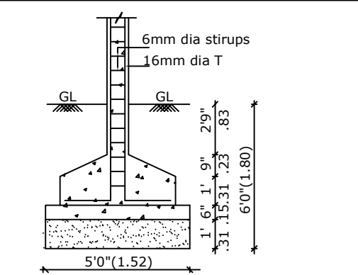
COLUMN FOUNDATION DETAIL
